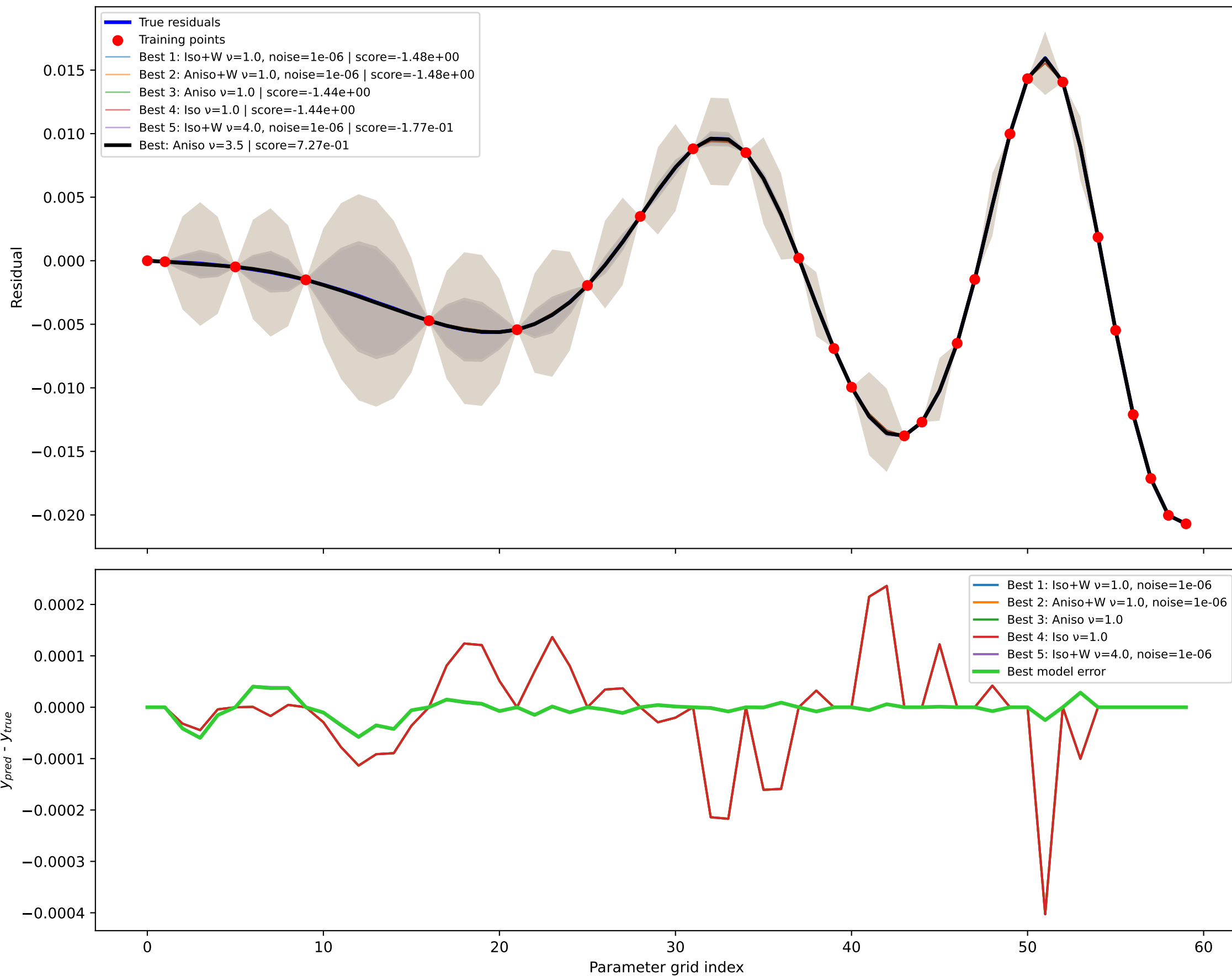
GPR kernel comparison node=13 RMSE=1.841e-05, train RMSE=2.126e-11
